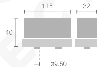
Cut-Out Dia : Ø10.5mm All Dimensions are in mm.*
